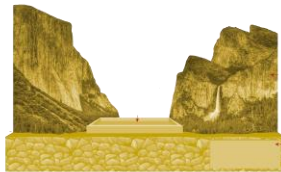
Superstate Base =
